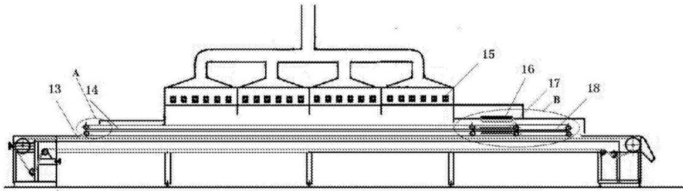
Schematic diagram of tea cylinder microwave water-removing machine
